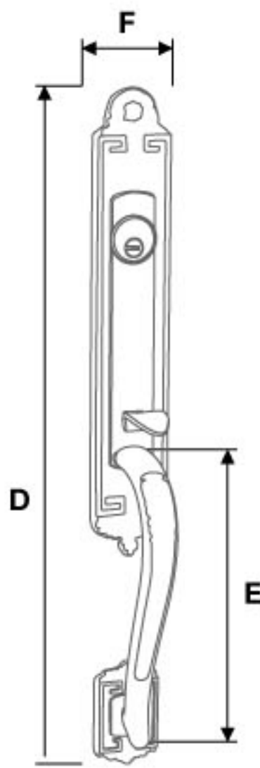
Front Plate Diagram for H1, H2
