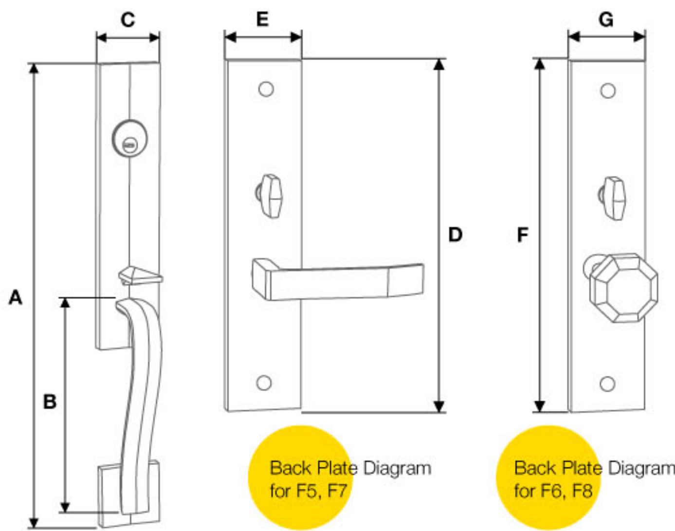
Front Plate Diagram for F5, F6, F7, F8
