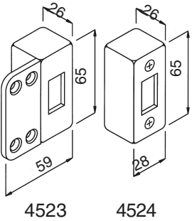
Keeps for inward opening doors.
