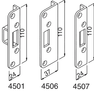
Striker plates for outward opening doors.
