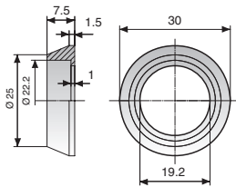
Protective collar 804757
