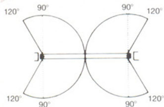
Center-Hung Inward and Outward Opening (90° Hold-Open)
