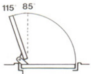
Offset-Hung 115° One-Side Opening Right or Left Hand (85° Hold-Open)
